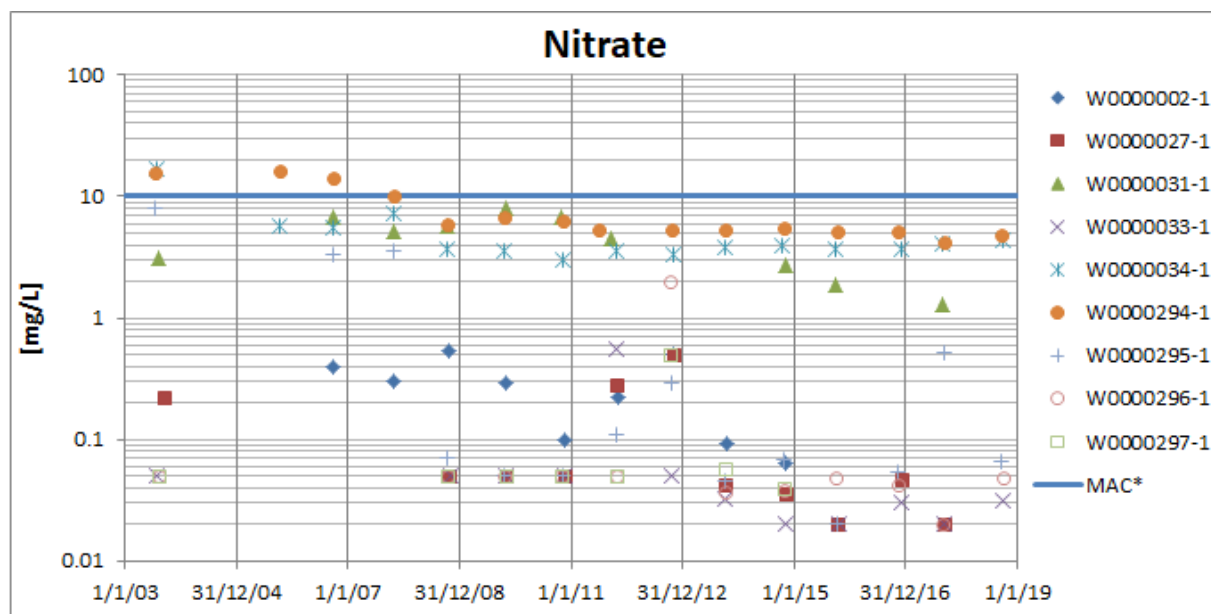
Chart 4.5 Nitrate concentrations in PGMN wells
