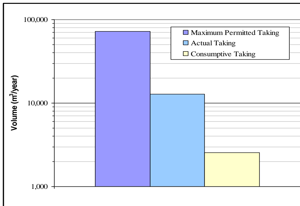
Figure 5.5 Annual permitted, actual, and consumptive water taking for the Greenville municipal water supply
