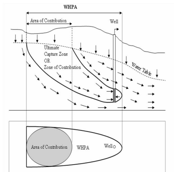
Figure 6.9 Conceptualization of capture zone, wellhead protection area, and area of contribution (modified from Franke et al.
