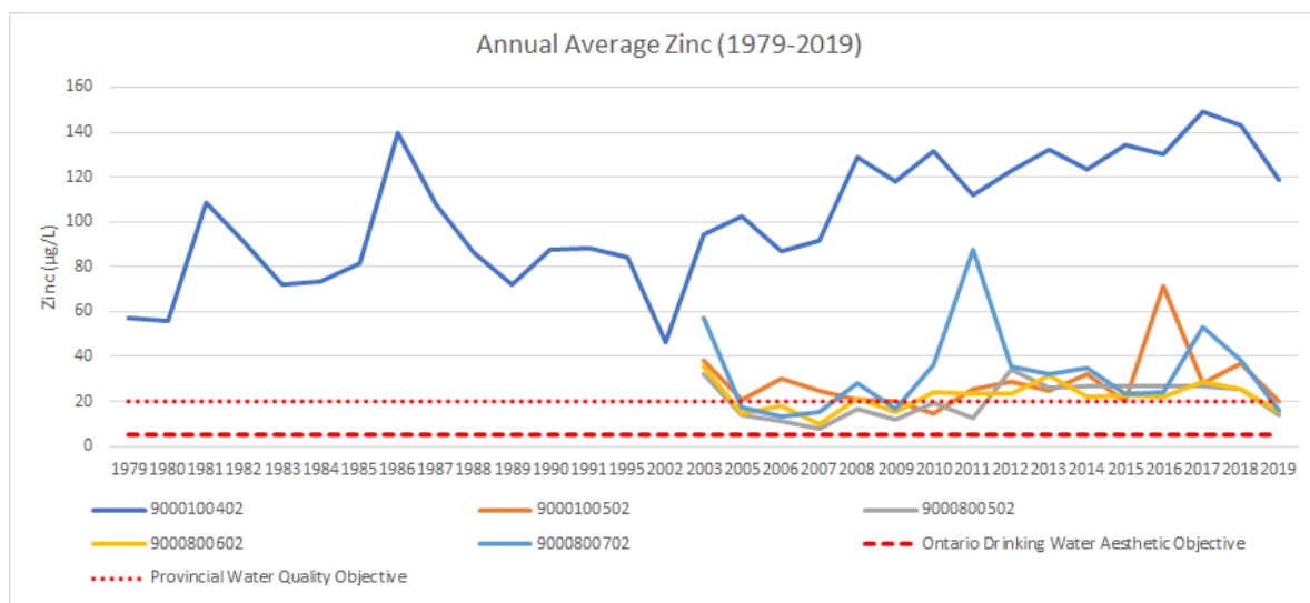
Chart 4.1 Zinc 4.1 Zinc concentrations at PWQMN stations
