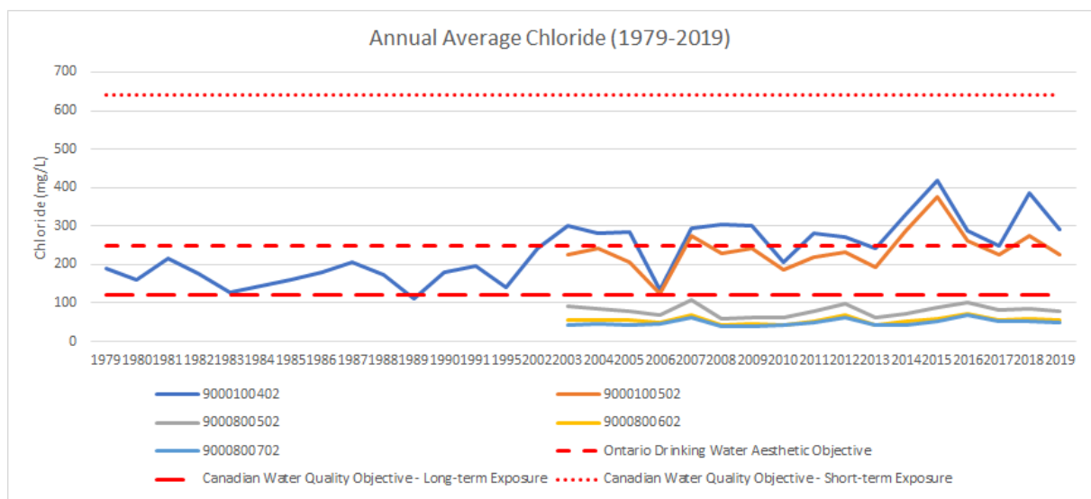
Chart 4.3 Chloride concentrations at PWQMN stations
