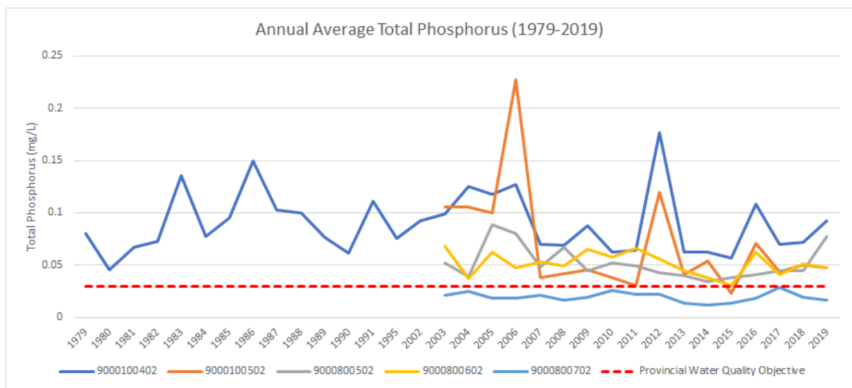
Chart 4.2 Total Phosphorus concentrations at PWQMN stations
