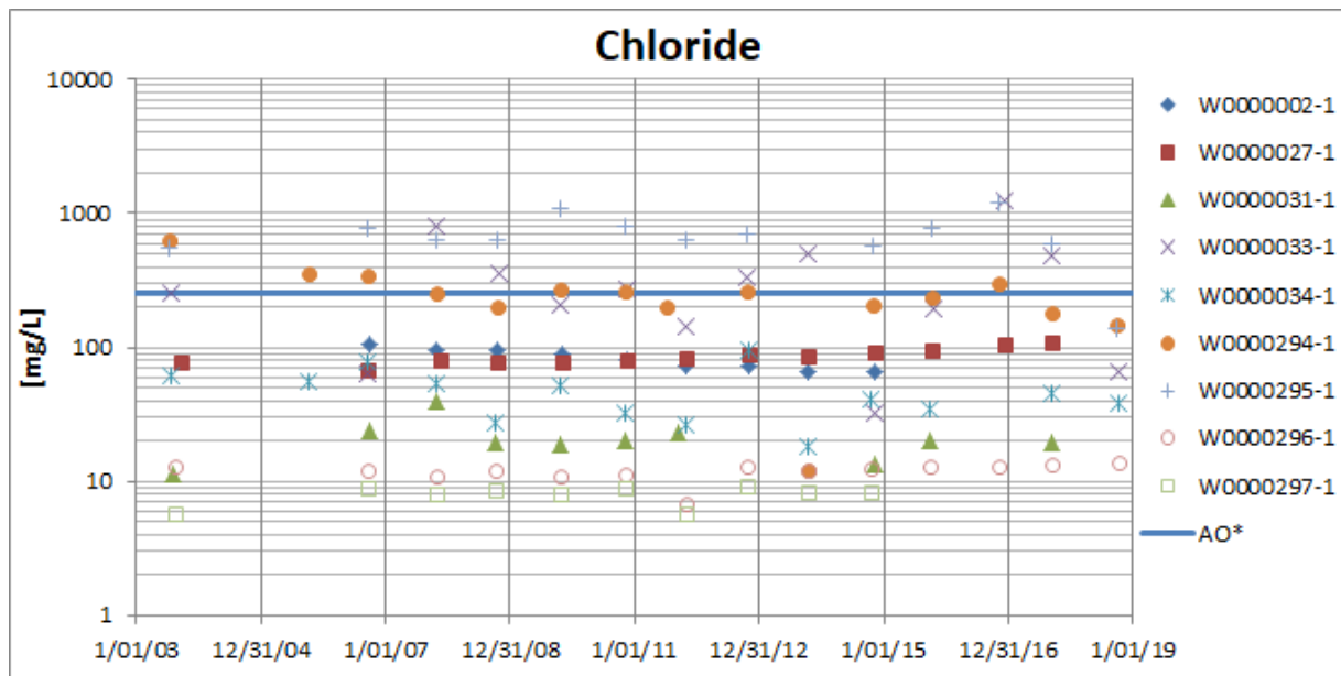
Chart 4.4 Chloride4.4 Chloride concentrations in PGMN wells
