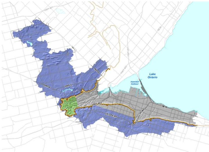
Figure 6.6 Significant Groundwater Recharge Areas – analysis areas. Urban area – grey; below escarpment – green; above escarpment – blue.
