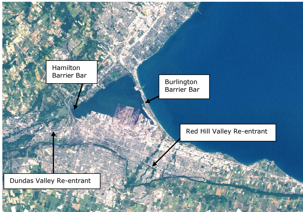
Barrier bars and re-entrants (Landsat 7 Orthorectified Imagery over Canada, Level 1, 1999)
